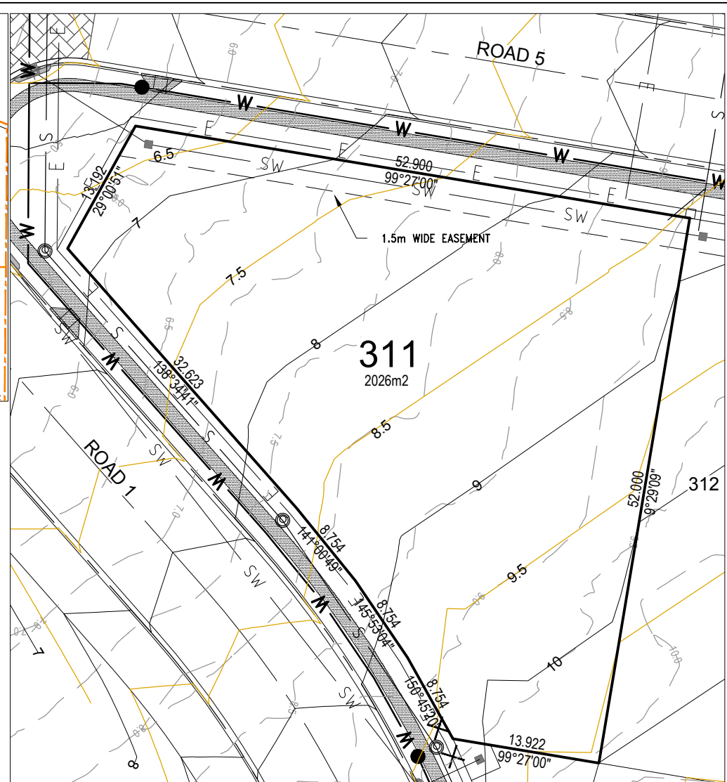
LOT 311 Scale 1:500
